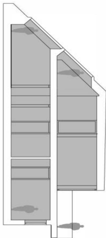
REZ / SECTION
